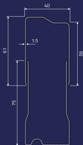
FASCIA MOD. 01
