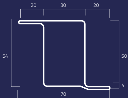
F26C
