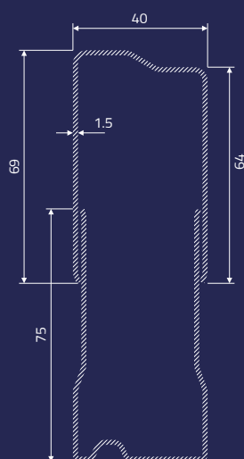
FASCIA MOD. 08
