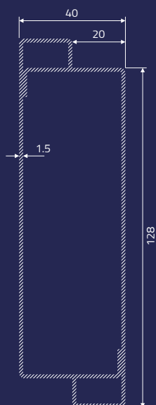
FASCIA MOD. 04
