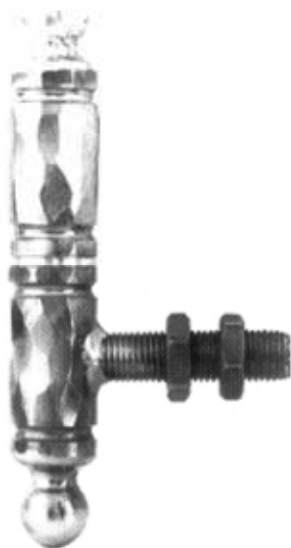
Art. 134B01 Filetto 14 MA H 120 mm Art. 134B02 Filetto 18 MA H 175 mm Art. 134B03 Filetto 22 MA H 230 mm
