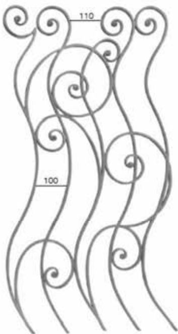
Art. 308A01 \square 14 x 8 mm H 1000 L 535 mm
