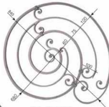
Art. 308A08 \square 14 + \square 14 x 8 mm H 680 L 840 mm
