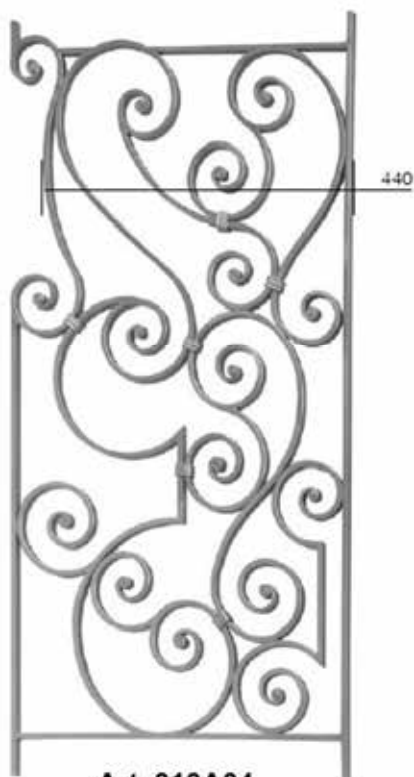
Art. 313A04 □ 14 x 8 mm H 1000 mm L 485 mm
