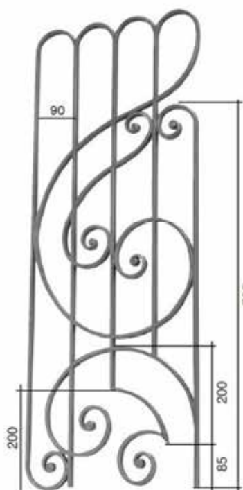
Art. 313A07 □ 14 x 8 mm H 1000 mm L 385 mm
