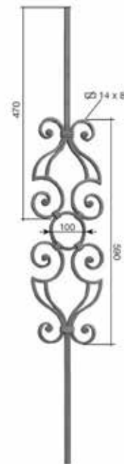
Art. 306A04 □ 14 mm H 1000 L 205 mm
