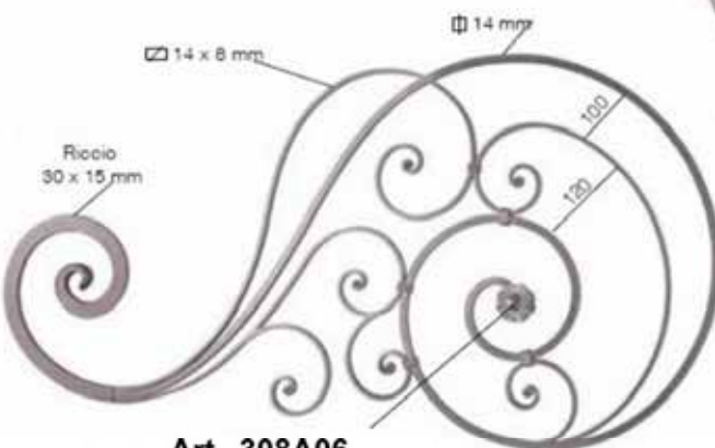
Art. 308A06 \square 14 + \square 14 x 8 mm H 700 L 1360 mm
