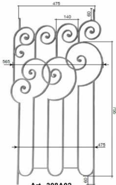
Art. 308A02 \square 14 x 8 mm H 1000 L 580 mm
