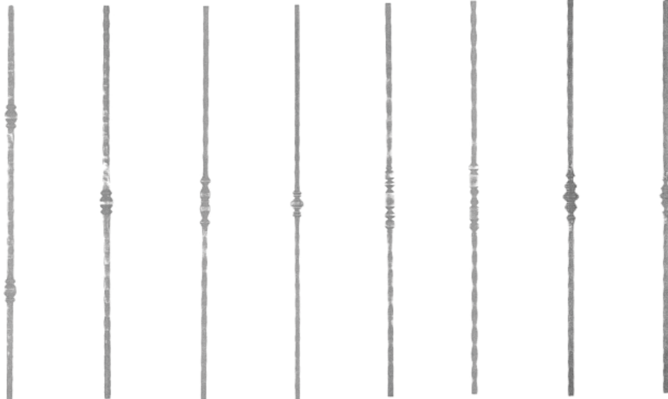
Art. 146B01 Art. 146B02 Art. 146B03 Art. 146B04 Art. 146B05 Art. 146B06 Art. 146B07 Art. 146B08 ∅ 12 mm ∅ 12 mm ∅ 12 mm ∅ 12 mm ∅ 12 mm ∅ 12 mm ∅ 12 mm ∅ 12 mm H 1000 mm H 1000 mm H 1000 mm H 1000 mm H 1000 mm H 1000 mm H 1000 mm H 1000 mm
