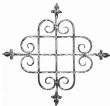
Art. 86A04 Ø 14 mm 850x850 mm
