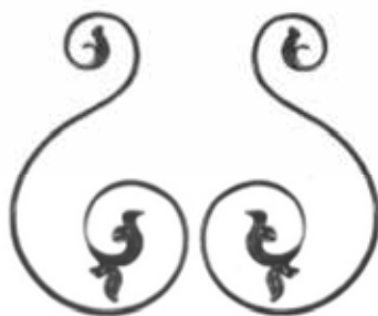
Art. 80A03 □16x8 260x450mm Art. 80A04 □16x8 260x450mm
