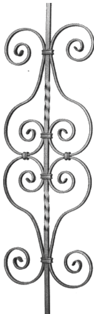
Art. 38A03 \phi 12 \nabla 12 \times 6 \text{ mm} Art. 38A04 \phi 14 \nabla 14 \times 6 \text{ mm} 275 x 900 mm
